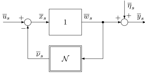
Fig. 2. Steady-state behaviour of the block-structured nonlinear feedback system.
